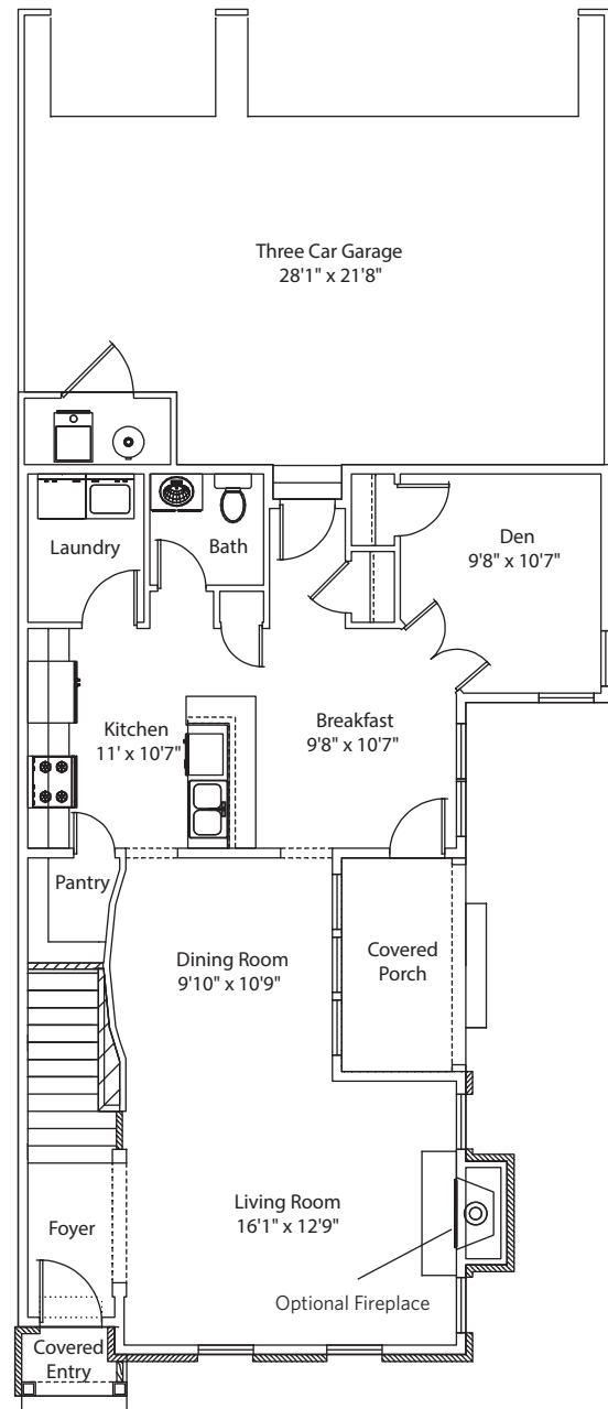
Main Floor
